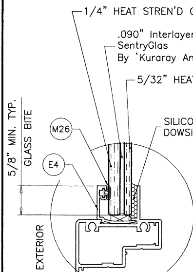
GLASS TYPE 'AA'
